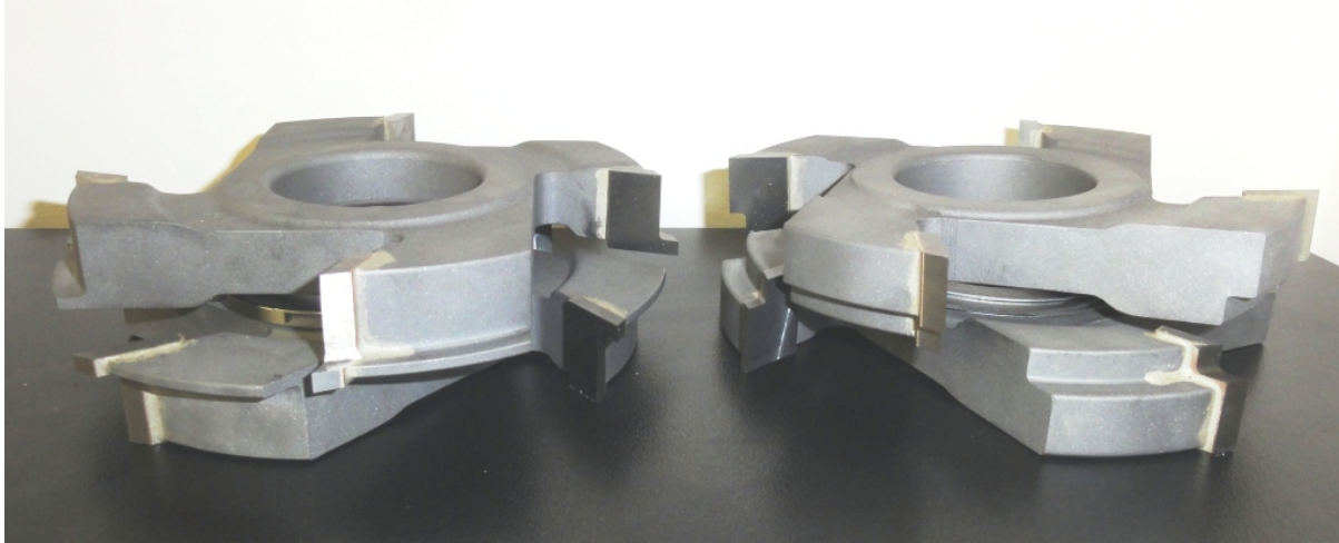
Set of 2: 4 wing x 4 wing TCT interlocking shim adjustable Flooring cutters
