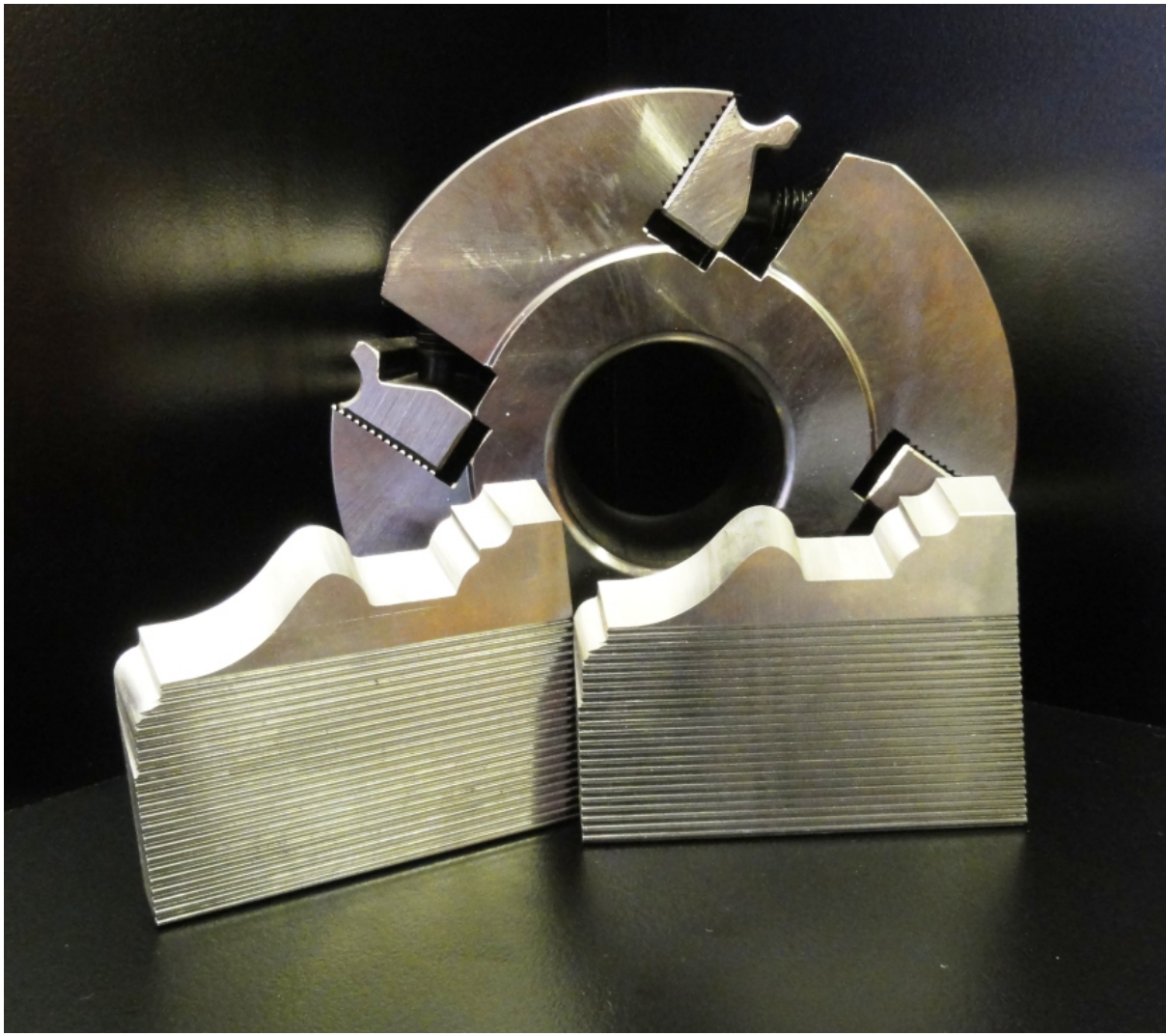
HSS and TCT Serrated Back Profile Blades
